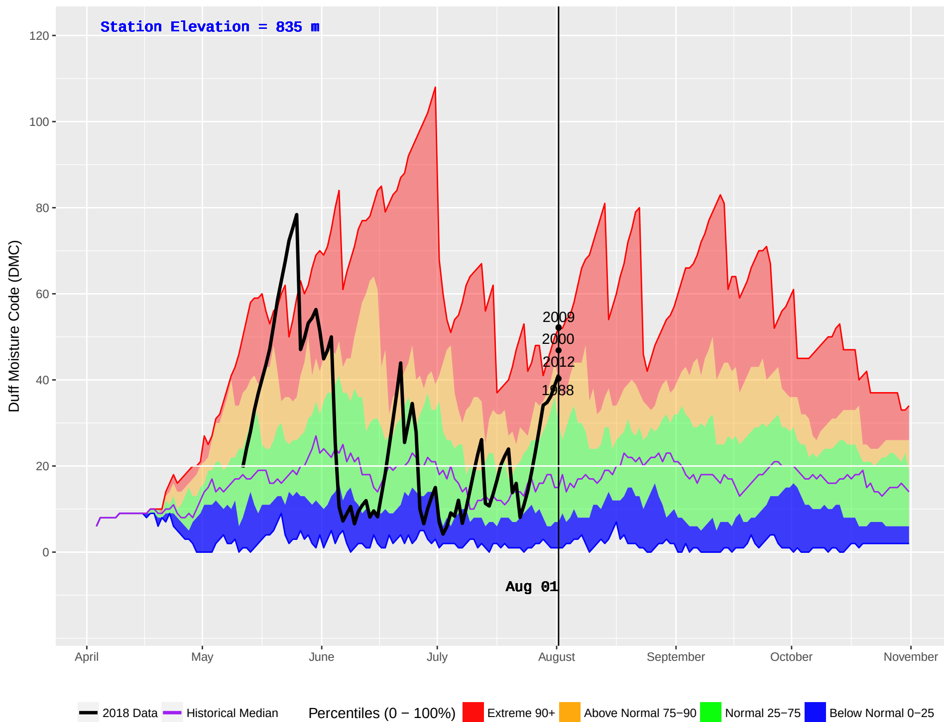
SILVER (120) : Historical (1986–2016) and Current (2018) Daily Duff Moisture Code (DMC)
