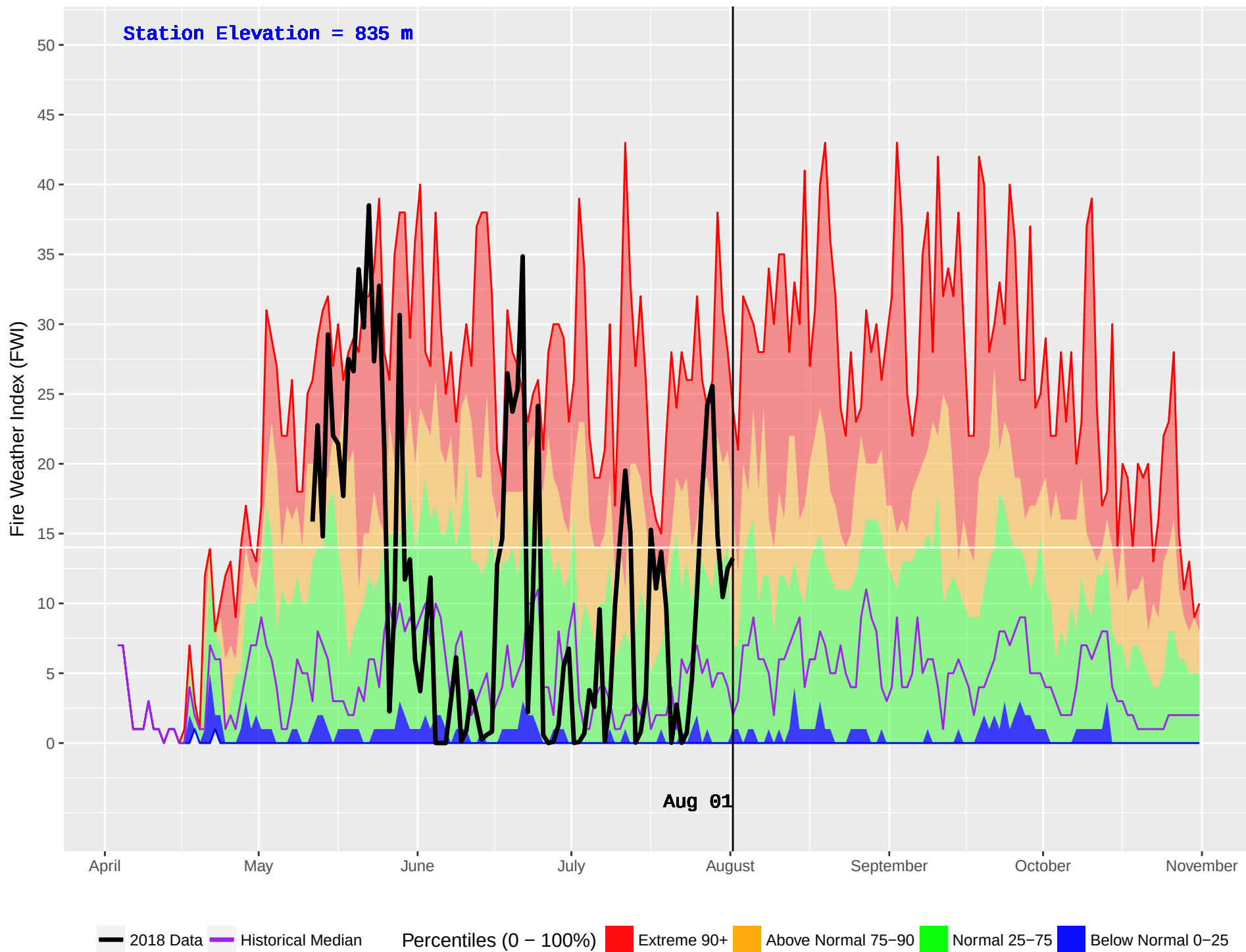
SILVER (120) : Historical (1986–2016) and Current (2018) Daily Fire Weather Index (FWI)
