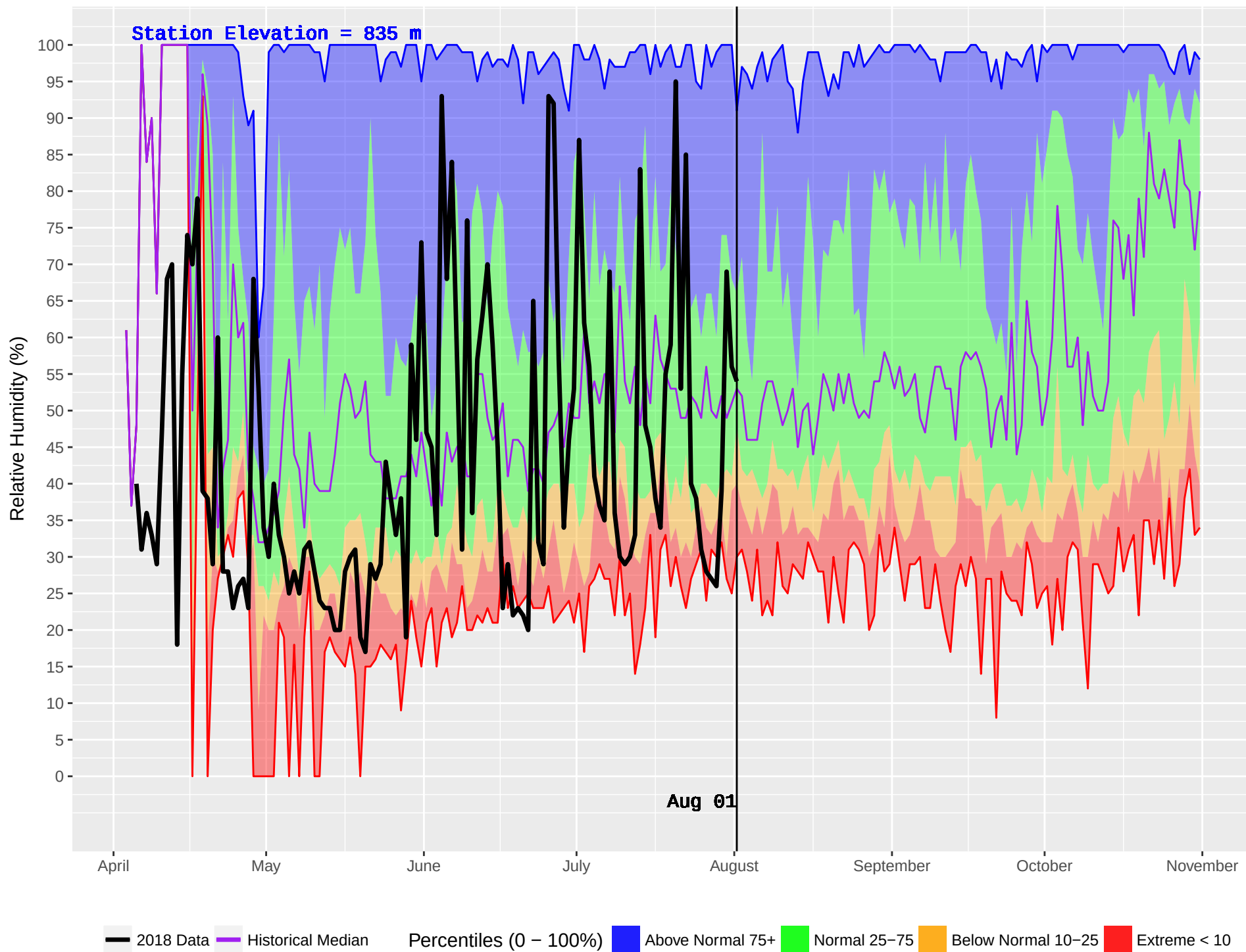
SILVER (120) : Historical (1986–2016) and Current (2018) Daily Relative Humidity
