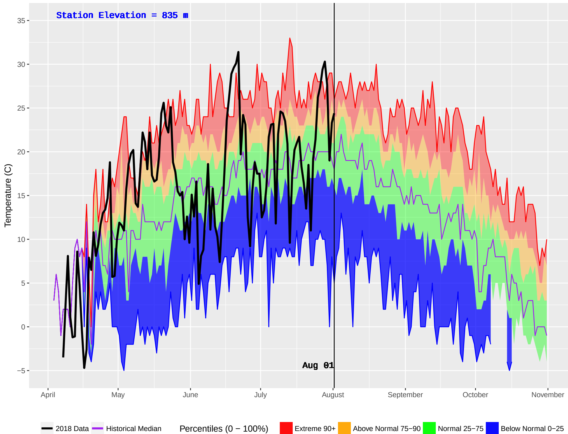
SILVER (120) : Historical (1986–2016) and Current (2018) Daily Temperature
