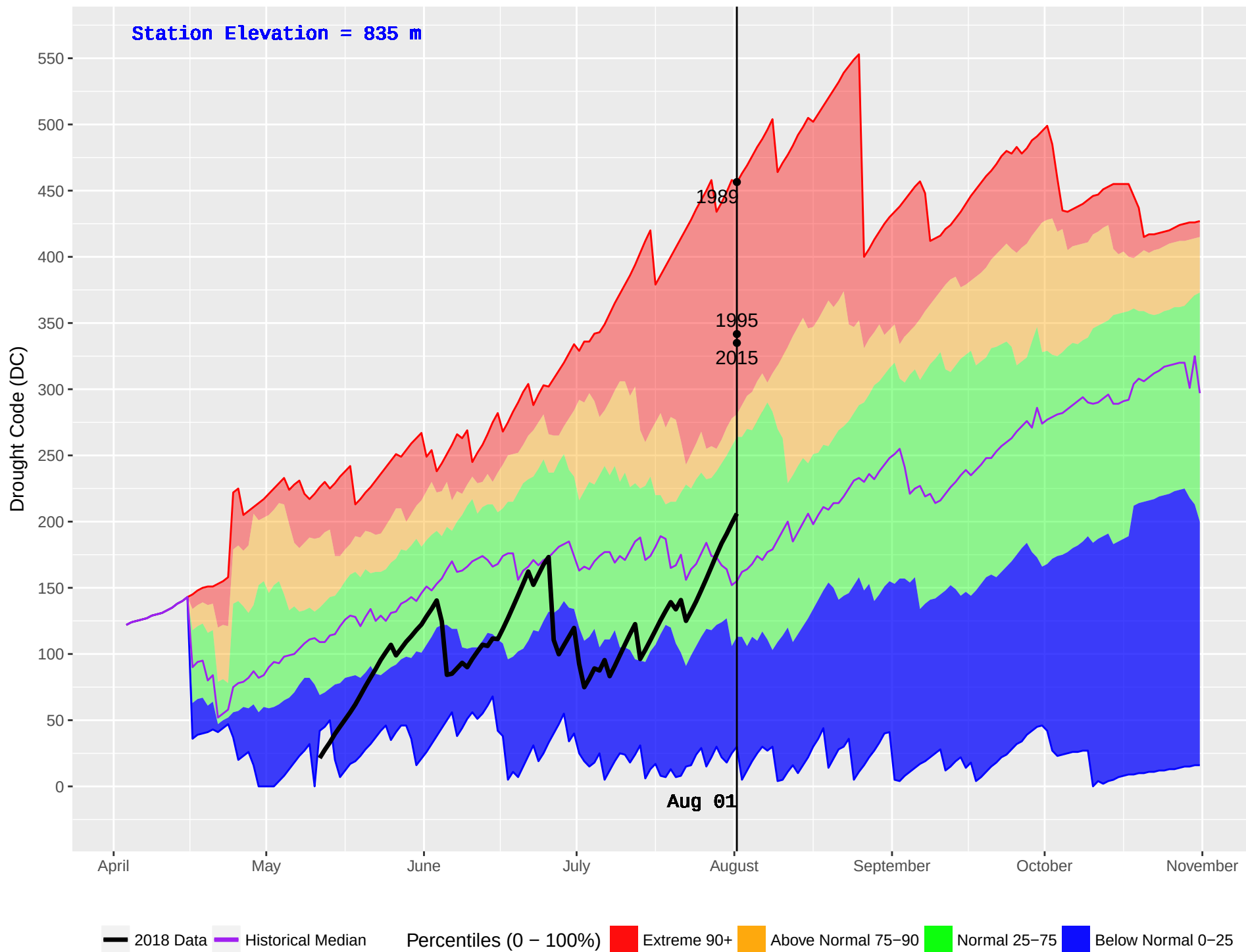
SILVER (120) : Historical (1986–2016) and Current (2018) Daily Drought Code (DC)
